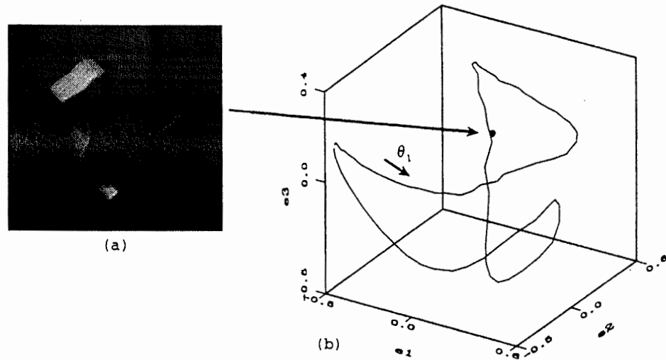
Figure 3: (a) An input image. (b) The input image is mapped to a point in the object eigenspace. The location of the point on the parametric curve determines the pose of the object in the input image.
