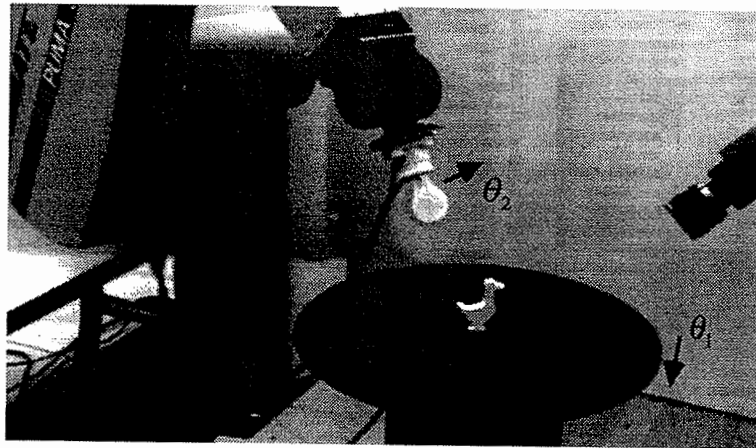
Figure 1: Setup used for automatic acquisition of object image sets. The object is placed on a motorized turntable.
