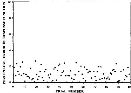
Figure 3: The percentage average error between actual and estimated response curves for the 100 synthetic trials. The maximum error was found to be 2.7%.
