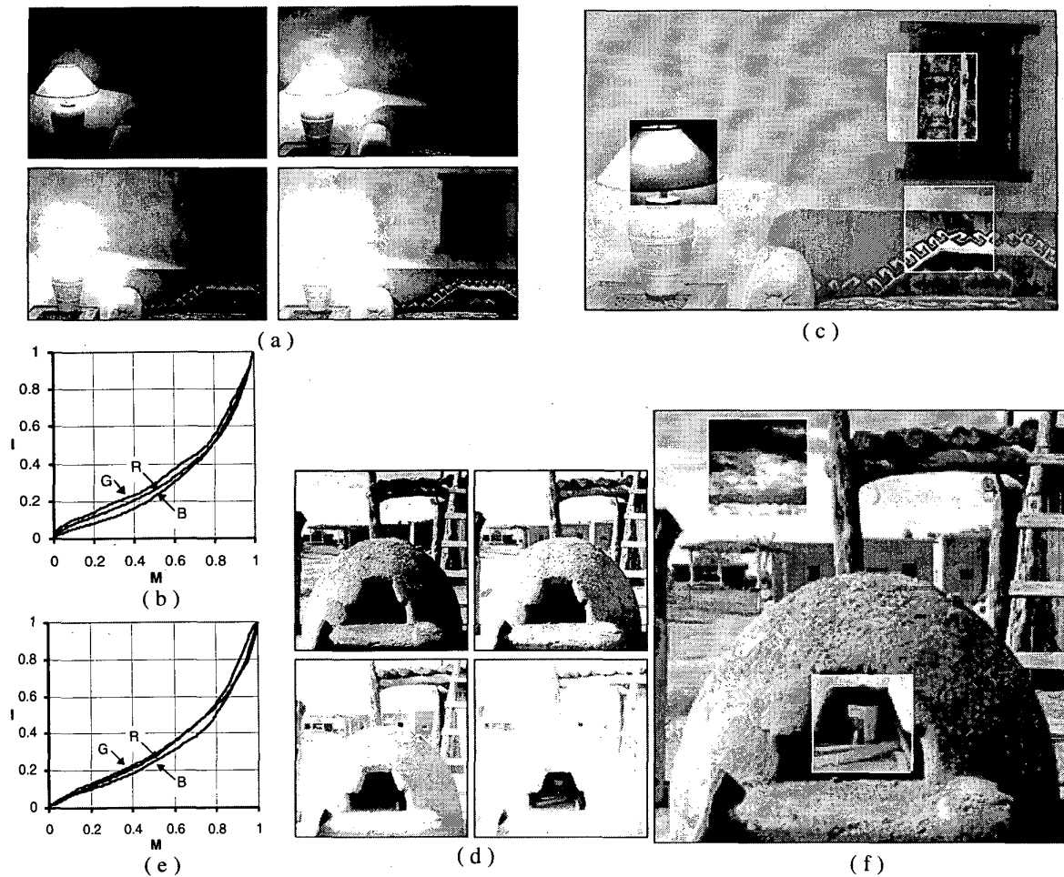
Figure 7: Self-calibration results for color slides taken using a Nikon 2020 photographic camera. The slides are taken using film with ISO rating of 200 in (a) and 100 in (d). Response functions are computed for each color channel and are shown in (b) and (e). The radiance images in (c) and (f) are histogram equalized and the three small windows shown in each radiance image are locally histogram equalized. The details around the lamp and within the wooden window in (c) and the clouds in the sky and the objects within the clay oven in (f) illustrate the richness of visual information embedded in the computed radiance images.
