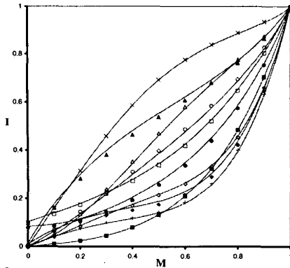
Figure 2: Self-calibration was tested using 100 randomly generated response functions. Here a few of the recovered (solid) and actual (dots) response functions are shown. In each case, four noisy test images were generated using random exposure ratios between image pairs in the range 0.45 \leq R \leq 0.55 . The initial ratio estimates were chosen to be 0.5.
