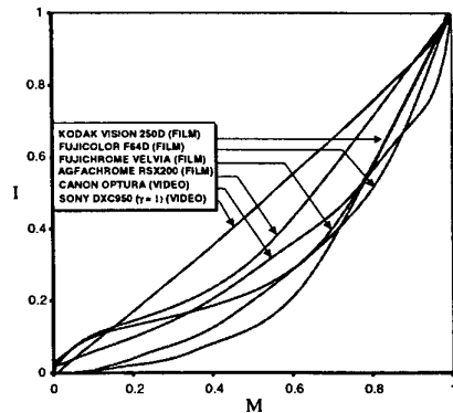
Figure 1: Response functions of a few popular films and video cameras provided by their manufacturers. These examples illustrate that a high-order polynomial may be used to model the response function.
