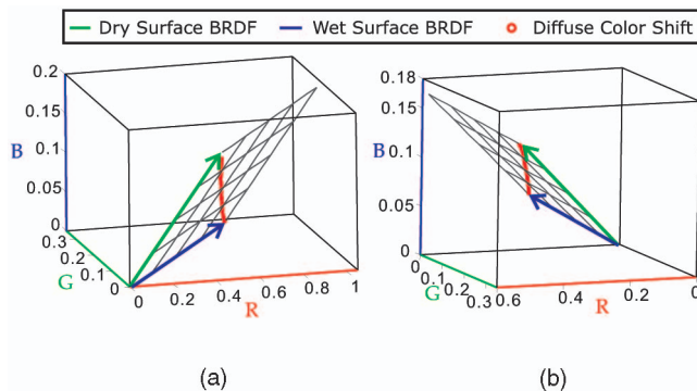
Fig. 11. All diffuse color shifts of wet materials are roughly straight lines connecting the BRDFs when fully dry and wet. (a) Orange cotton fabric. (b) Terracotta clay.
