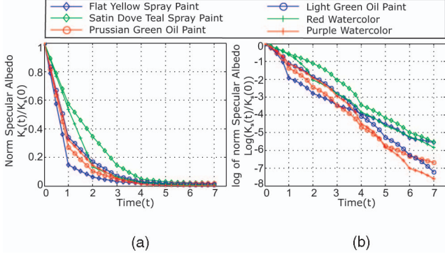
Fig. 7. (a) The falloff with time of K_s (normalized by the initial value K_{s,wet} ) of various paint samples. (b) This plot is similar to the one in (a), except that the dry value is first subtracted and then the natural log is applied. Note that K_s in the case of paints attenuates exponentially with time.
