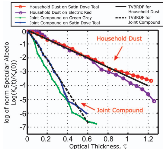
Fig. 20. The attenuation of K_s with time for both the dust measurements and its analytic TVBRDF model. Black lines are the TVBRDF models, whereas the marked color curves are the measurements. All curves are normalized and then plotted in the natural log space.
