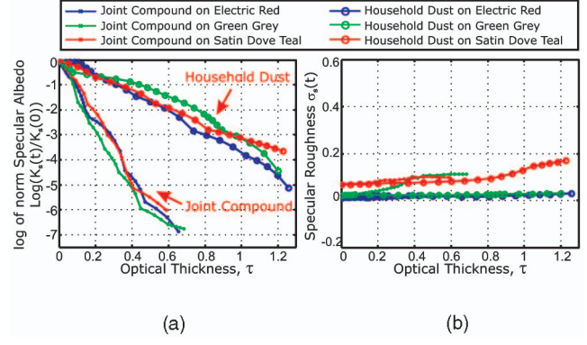
Fig. 14. (a) The natural log of K_s normalized by its initial value K_{s0} versus optical thickness \tau . It clearly shows that K_s decays exponentially with the optical thickness \tau and the slopes of the lines depend on the types of dust. (b) Absolute values of \sigma_s versus optical thickness \tau .
