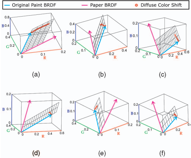
Fig. 9. The diffuse color shifts associated with drying paints lie on dichromatic planes spanned by the diffuse color vector of the surface (shown in magenta) and the diffuse color vector of the paint (shown in cyan). The first row shows the dichromatic planes for watercolors: (a) blue watercolor, (b) purple watercolor, and (c) red watercolor. The second row shows the dichromatic planes for oil paints: (d) cadmium yellow oil paint, (e) light green oil paint, and (f) Prussian red oil paint.
