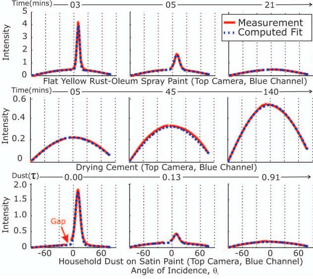
Fig. 5. Example fits for three of our acquired samples. Each row shows the measurement (red solid lines) obtained in the blue color channel of the top camera for three different time instances and the results of fitting appropriate analytic BRDF functions (blue dotted lines). Though the changes in BRDFs across time are dramatic, all our fits are found to be fairly accurate with a maximum RMS error of 3.8 percent. The small gap in the original measurement indicated by the red arrow (around the incidence angle of 12 degrees) is due to the occlusion of the sample by the light source. However, because the sample plane is tilted, the occlusion is shifted away from the peak of the specular lobe and does not affect the robustness of the fitting.
