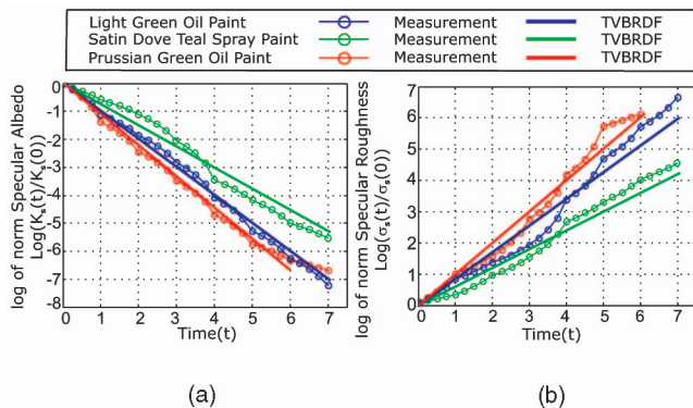
Fig. 18. The temporal variation of (a) K_s and (b) \sigma_s of both the paint measurements and their analytic TVBRDF model. Curves of the same material have the same color, but with markers to distinguish the measurements and the TVBRDF model. All curves are normalized and then plotted in the natural log space.
