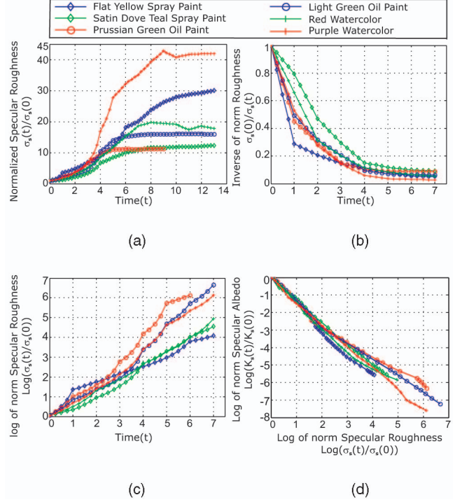
Fig. 8. (a) \sigma_s (normalized by the initial value \sigma_{s,wet} ), plotted as a function of time for several of the paint samples and can be seen to vary exponentially, (b) 1/\sigma_s (normalized by the initial value \sigma_{s,wet} ), plotted as a function of time, (c) 1/\sigma_s , plotted with a negative natural log scale after 1/\sigma_{s,dry} is subtracted, and (d) linear relation observed between the log of the normalized K_s and \sigma_s .
