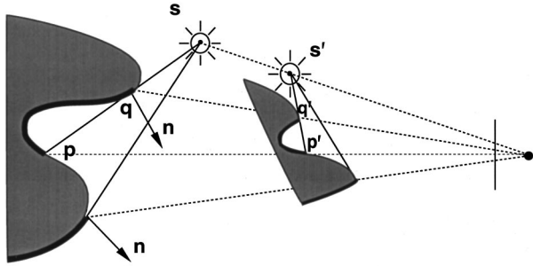
Fig. 2. In this 2-D illustration of the GPBR transformation, the lower shadow is an attached shadow, while the upper one is composed of both attached and cast components. A GPBR transformation has been applied to the left surface, yielding the right one. Note that under a GPBR, all surface points and the light source are transformed along the optical rays through the center of projection. Transforming the light source from \mathbf{s} to \mathbf{s}' preserves the shadows.
