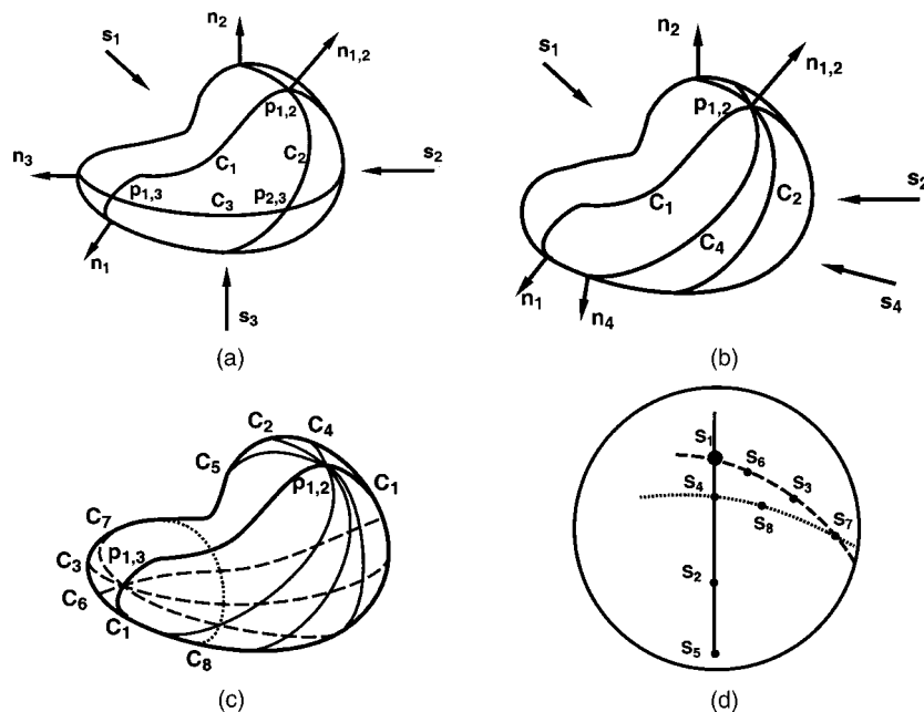
Fig. 6. Reconstruction up to a GBR from attached shadows. For a single object in fixed pose, these figures show superimposed attached shadow contours C_i for light source direction \mathbf{s}_i . The surface normal where C_i intersects the occluding contour is denoted by \mathbf{n}_i . The normal at the intersection of C_i and C_j is denoted by \mathbf{n}_{i,j} . (a) The three contours intersect at three points in the image. (b) The three contours meet at a common point, implying that \mathbf{s}_1 , \mathbf{s}_2 , and \mathbf{s}_3 lie on a great circle of the illumination sphere. (c) Eight attached shadow boundaries, of which four intersect at \mathbf{p}_{1,2} and four intersect at \mathbf{p}_{1,3} ; the direction of the light sources \mathbf{s}_1, \dots, \mathbf{s}_8 and the surface normals at the intersection points can be determined up to a GBR. (d) Structure of the illumination sphere S^2 for the light source directions generating the attached shadow boundaries in (c).
