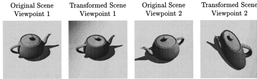
Fig. 1. Illustration of the effect of applying a generalized perspective bas-relief (GPBR) transformation to a scene composed of a teapot resting on a supporting plane. The first image shows the original teapot. The second image shows the teapot after having undergone a GPBR transformation (a_1, a_2, a_3, a_4) = (0.05, 0.05, 0.05, 1) with respect to the viewpoint used to generate the first image. Note that the attached and cast shadows as well as the occluding contour are identical in the first two images. The third image shows the original teapot from a second viewpoint. The fourth image reveals the nature of the GPBR transformation, showing the transformed teapot from the second viewpoint.
