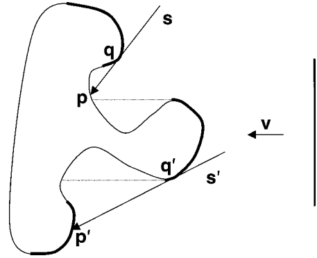
Fig. 5. Illustration of some of the ideas in the proof of Proposition 3.1. In two dimensions, consider the shadows of a non-convex object observed under orthographic projection with viewing direction \mathbf{v} . Over all light source directions, only points on the thickened arcs can fall on a visible global attached shadow boundary. The points between the thickened arcs and the dotted horizontal lines are visible to the observer, but there is no light source direction for which these points satisfy the global attached shadow conditions. Nonetheless, there exist light source directions for which each of these points can lie on a cast shadow boundary (e.g., \mathbf{p} lies on a cast shadow boundary for light source direction \mathbf{s} ). Since \mathbf{p} is a cast shadow, it lies in the tangent plane to an attached shadow point \mathbf{q} ; when the portion of the surface about \mathbf{q} is transformed by a GBR transformation, \mathbf{p} must also be transformed by the same GBR transformation. Similarly, points such as \mathbf{p}' and \mathbf{q}' are, respectively, cast and attached shadow points for light source \mathbf{s}' . Note that \mathbf{p}' can also be an attached shadow boundary point. Because \mathbf{p}' lies in the tangent plane to \mathbf{q}' , the same GBR that is applied to \mathbf{q}' and its tangent plane must be applied to \mathbf{p}' . Hence the two thickened arcs containing \mathbf{p}' and \mathbf{q}' must be transformed by the same GBR if they are to be strongly shadow equivalent.
