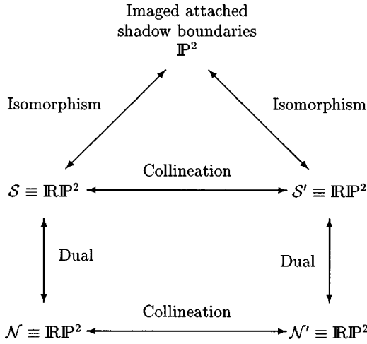
Fig. 4. Relation of different spaces in the proof of Proposition 3.1.
