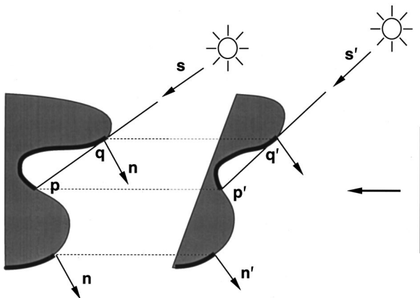
Fig. 3. Under orthographic projection, the image points that lie in shadow for a surface under light source \mathbf{s} are identical to those in shadow for a transformed surface under light source \mathbf{s}' . In this 2-D illustration, the lower shadow is an attached shadow, while the upper one is composed of both attached and cast components. A generalized bas-relief (GBR) transformation with both flattening and an additive plane has been applied to the left surface, yielding the right one.
