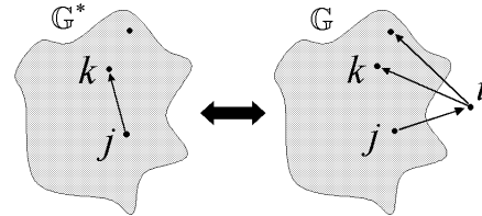
Fig. 14. Edge Splitting - directed case.
