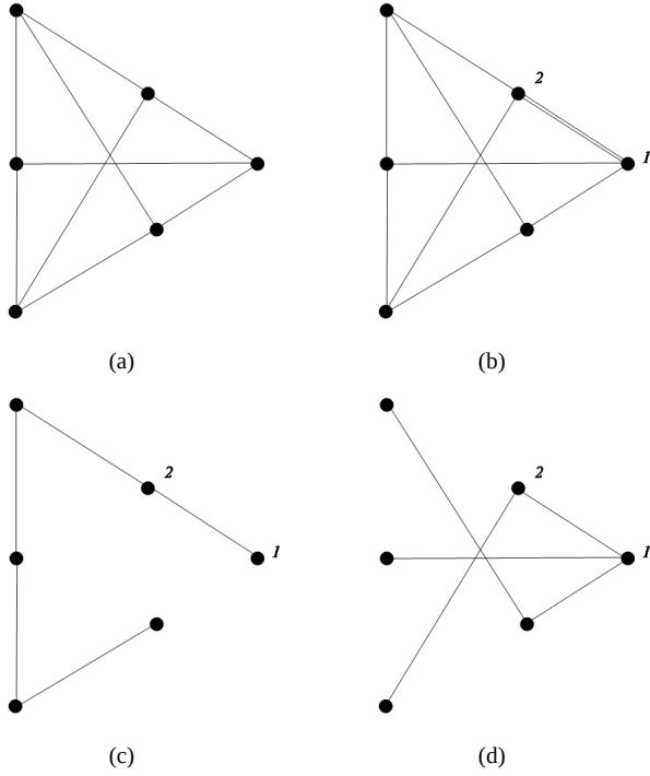
Fig. 21. A minimally rigid point formation is shown in (a). The graph with the double edge (2, 1) is shown in (b). The global leader is labeled with 1 and the first follower is labeled with 2. The graph in (b) can be partitioned into two spanning trees as shown in (c) and (d).
