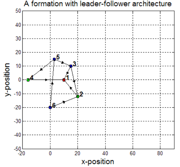
Fig. 9. A flexible formation is shown. It does not satisfy the conditions given in 3.3, i.e., the underlying undirected graph is flexible. The agent of out-degree 0 (global leader) is depicted with color red and has index 1. The agents of out-degree 1 are depicted with green and have indices 2 and 4. The agents of out-degree 2 are depicted with color blue and have indices 3, 5, and 6.
