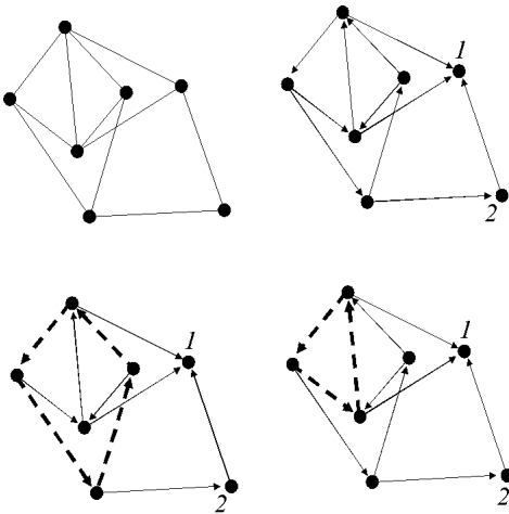
Fig. 26. Given the point formation shown top left, if the global leader labeled with 1 and the first follower labeled with 2 are chosen as shown on top right, then we obtain a cyclic rigid formation. Cycles are shown on bottom right and bottom left with dotted edges. This selection of global leader-first follower pair results in only cyclic formations, and does not permit any acyclic formations.
