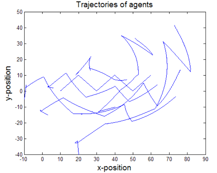
Fig. 19. Trajectories of agents in the formation shown in Figure 18.
