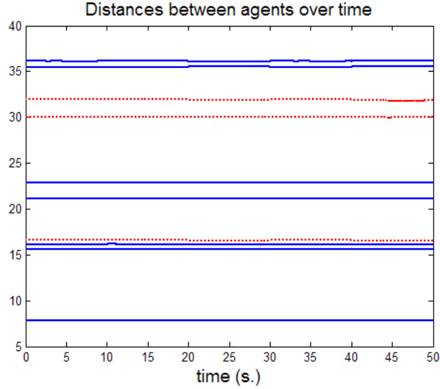
Fig. 8. Distances between agent pairs (of the formation shown in Figure 6) are shown over time as the global leader moves. The blue solid lines show the distances between agents where there exist links between those pairs. The red dotted lines show the distances between agent pairs where there are no links between those pairs.
