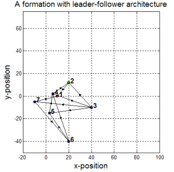
Fig. 18. A rigid formation created by vertex addition and edge splitting. The agent of out-degree 0 (global leader) is depicted with color red and has index 1. The agent of out-degree 1 is depicted with green and has index 2. The agents of out-degree 2 are depicted with color blue and has indices 3, 4, 5, 6, 7.
