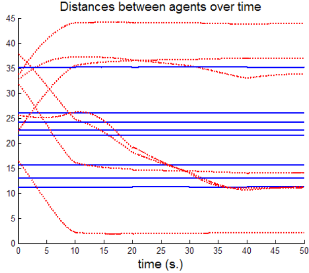
Fig. 11. Distances between agent pairs (of the formation shown in Figure 9) are shown over time as the global leader moves. The blue solid lines show the distances between agents where there exist links between those pairs. The red dotted lines show the distances between agent pairs where there are no links between those pairs.
