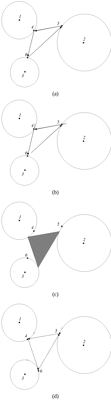
Fig. 17. (a) This figure shows the distance constraints that need to be satisfied by agents 4, 5, and 6 of the formation shown in Figure 16. The points in this figure clearly satisfy the constraints; (b) If noise is added to the lengths of links that lie on the 3-cycle (4, 6, 5, 4) , then points p_4 , p_5 , and p_6 fail to satisfy the distance constraints at their current positions; (c) The new distance constraints corrupted with noise can be represented by a triangle. It can be seen that the triangle can be placed between the circles in such a way that its vertices touch the circles at one single point, thus satisfying the distance constraints. (d) The vertices of this triangle determine the new locations of points p_4 , p_5 , and p_6 as shown with filled circles. The previous positions of the points are shown with empty circles.
