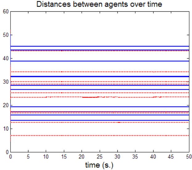
Fig. 20. Distances between agent pairs (of the formation shown in Figure 18) are shown over time as the global leader moves. The blue solid lines show the distances between agents where there exist links between those pairs. The red dotted lines show the distances between agent pairs where there are no links between those pairs.
