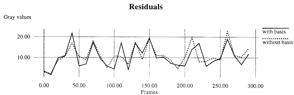
Figure 3: Above, excerpts from a sequence of tracked images. The white frames represent the region tracked by the SSD algorithm using an illumination basis, and black frames represent the regions tracked by an algorithm which does not. In some cases the estimates are so close that only one box is visible. Middle row, the region within the frame warped by the current motion estimate. Below, the residuals, in gray-scale units per pixel of the algorithms as a function of time.
