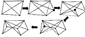
Fig. 4. A sequence for generating a globally rigid formation. The sequence starts with K_4 , and a new vertex (shown as a larger circle) is adjoined at each step by edge splitting operation. Edges about to be split are shown as dashed lines.
