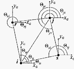
Fig. 8. The same point formation drawn with bearing constraints in the global coordinate system.
