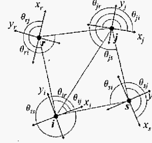
Fig. 7. A point formation with bearing constraints.
