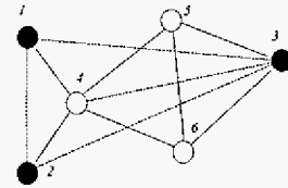
Fig. 6. The grounded graph shown with the additional inserted implicit edge (3, 4) .
