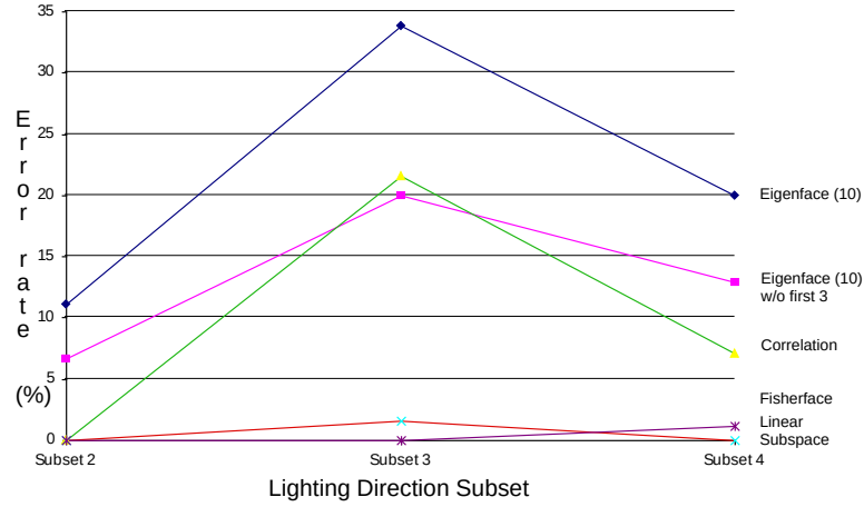
Fig. 4. Interpolation: When each of the methods is trained on images from both near frontal and extreme lighting (Subsets 1 and 5), the graph and corresponding table show the methods' relative performance under intermediate lighting conditions.
