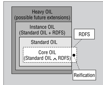
Figure 3. OIL's layered language model.
