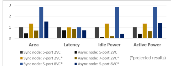
Fig. 4. Asynchronous and synchronous router comparison
