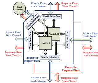
Fig. 1. Node structure for proposed asynchronous double-plane router
