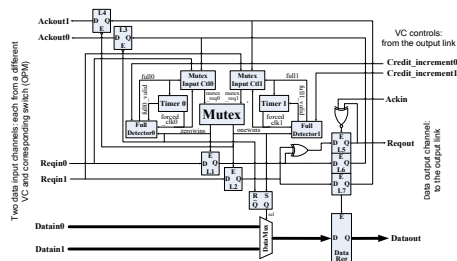
Fig. 2. Proposed VC control for an output channel interface
