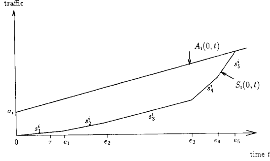
Fig. 7. Session i arrivals and departures after 0, the beginning of a system busy period.
