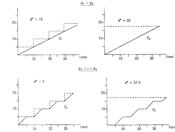
Fig. 2. The effect of increasing \phi_i for a steady session i .
