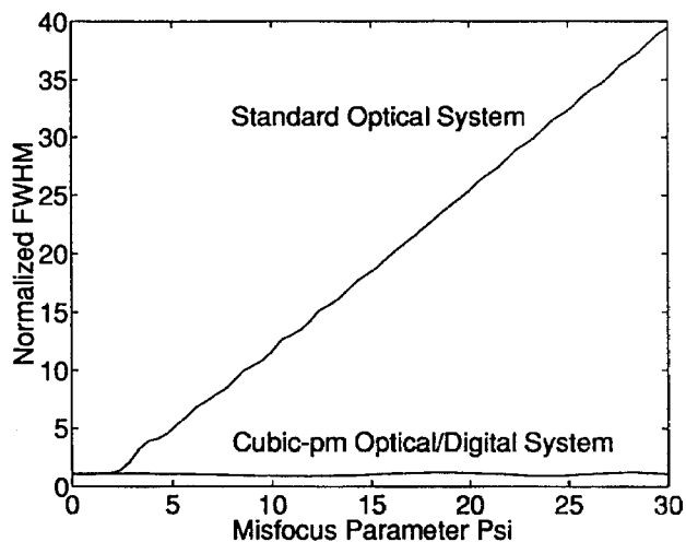
Fig. 7. Normalized full width at half-maximum amplitude (FWHM) of the PSF of the cubic-pm optical-digital system with comparison to that of the standard optical system.
