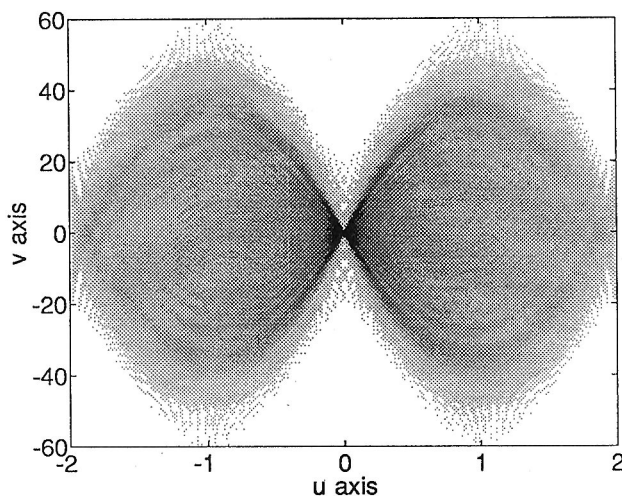
Fig. 3. Magnitude of the ambiguity function of the cubic-pm function with \alpha = 90 . Radial lines through this function are insensitive to angle for a broad range of angles.
