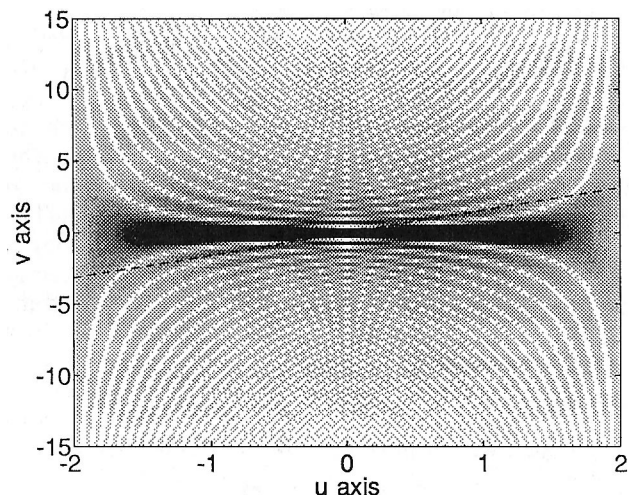
Fig. 1. Ambiguity function of a rectangular aperture. The radial line has a slope of \pi/2 , corresponding to an OTF with misfocus \psi = \pi^2/2 .
