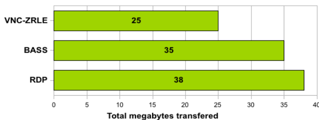
Figure 7. Web browsing performance
