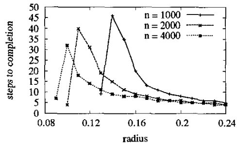
Fig. 9. Required steps for algorithm completion.
