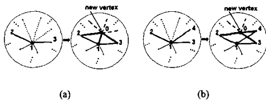
Fig. 1. (a) Vertex 3-split on two edges. Edges which are shifted to the new vertex 0 are shown with dashed edges, and new edges after split are shown with wider edges. (b) Vertex 3-split on three edges. Edges which are shifted to the new vertex 0 are shown with dashed edges, and new edges after split are shown with wider edges.
