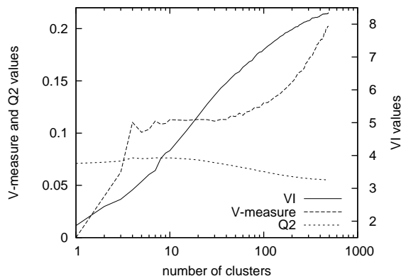
Figure 5: Results of pitch accent clustering measured by V-Measure, VI and Q_0
