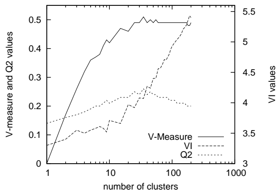
Figure 4: Results of document clustering measured by V-Measure, VI and Q_2
