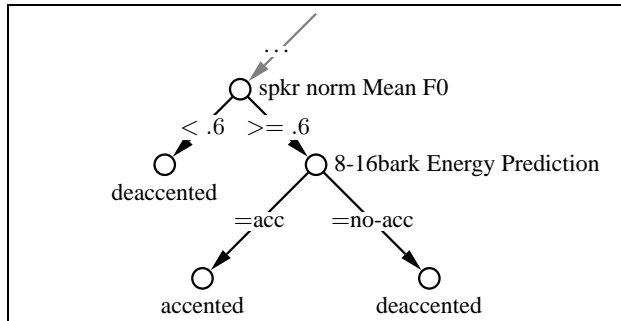
Figure 1: Detail view of single pitch-based classifier
