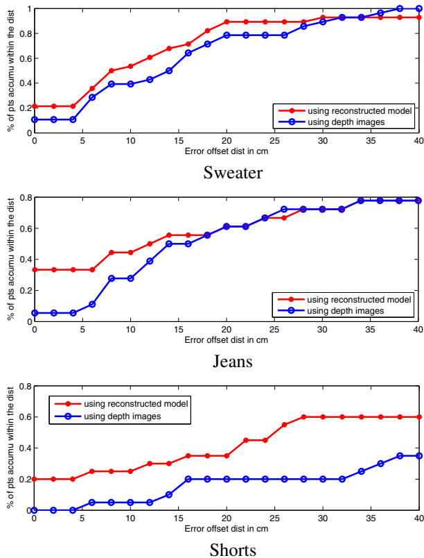
Fig. 6. Quantitative comparison of the proposed method (using reconstructed model) and our previous method (using individual depth images) [14]. The x axis is the Geodesic Error, and the y axis is the percentage of the input grasping points which give Geodesic Error smaller than the corresponding x . The results of a sweater, a pair of jeans, and shorts are shown from top to bottom, with maximum distance between any grasping points as 75cm, 65cm, and 55cm respectively.
