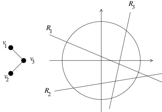
Figure 1: System of lines for a three-vertex graph.
