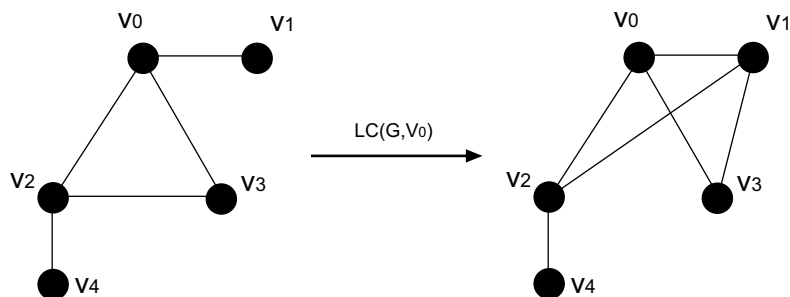
Figure 1: Local complementation.
