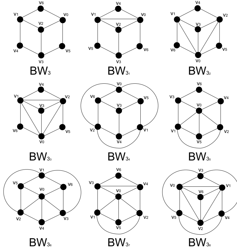
Figure 7: Family F_{BW_3} .
