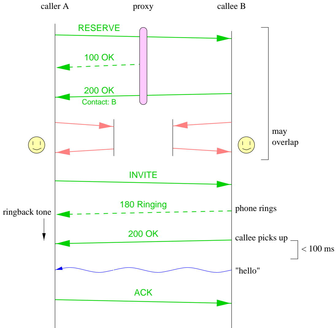
Figure 4: Two-phase setup with RESERVE request
