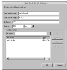
Figure 14: Telling Quartus about a new test bench
