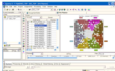
Figure 3: Assigning Pins Graphically
