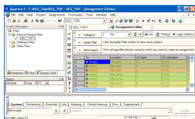
Figure 2: Assigning Pins Textually
