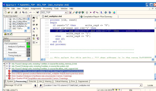
Figure 6: Diagnosing errors
