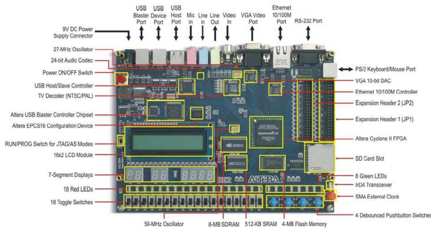
Figure 1: The Altera DE2 board
